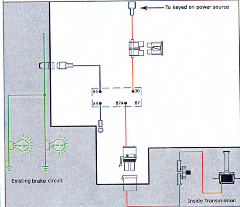
Normal Kit Diagram
