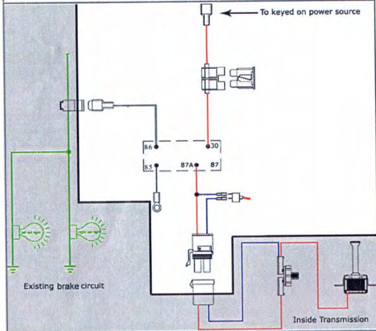
Kit with Towing Option
