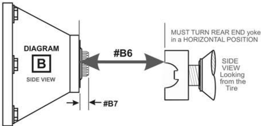
Typical FORD, DANA, some GM and some DODGE with TAB style yokes
