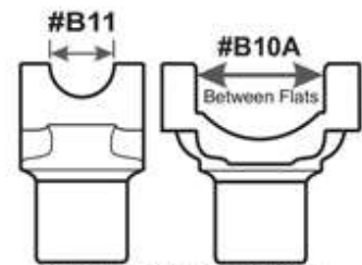
Typical STOCK GM and DODGE with inside clips
